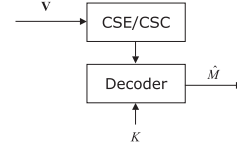
Figure 3: Hierarchical CSE-CSC-decoding.
