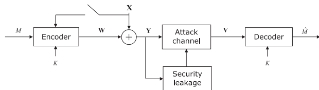
Figure 5: Attack design based on security leakages.
