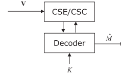
Figure 2: Iterative CSE-CSC-decoding.
